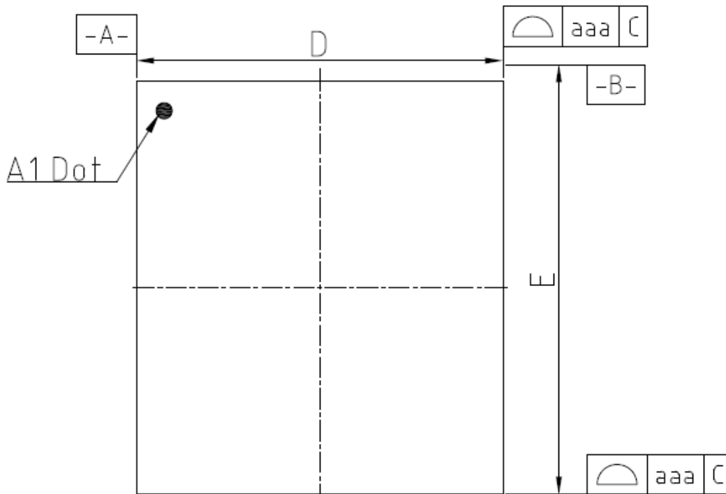
Figure 2 TOP View of Package
