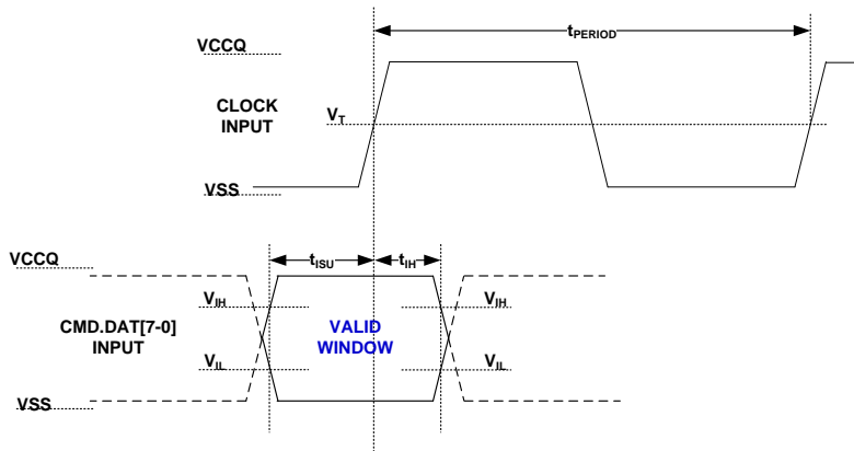
Figure 8 HS200 Device Input Timing
