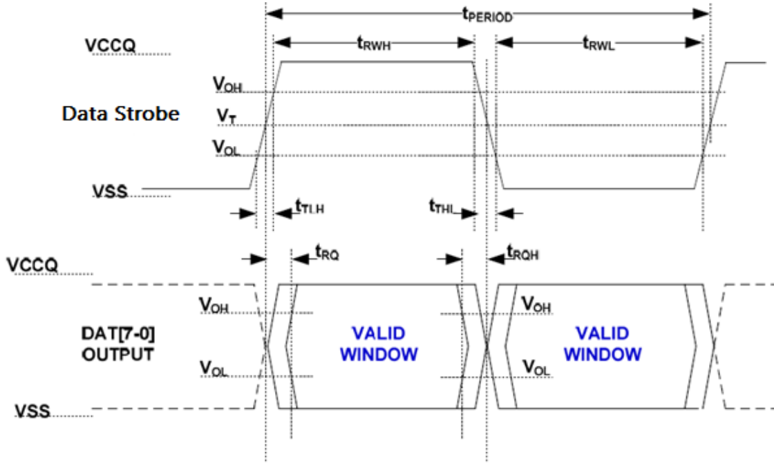
Figure 6 HS400 Device Output Timing
