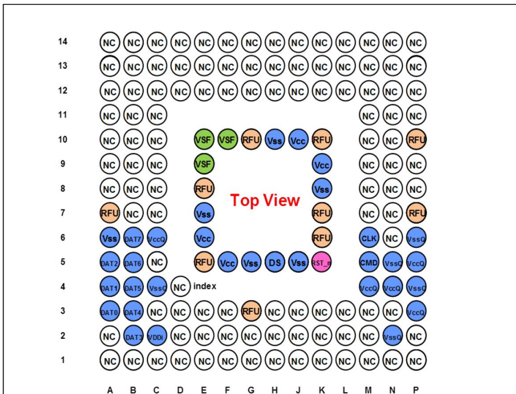
Figure 1 153 FBGA
